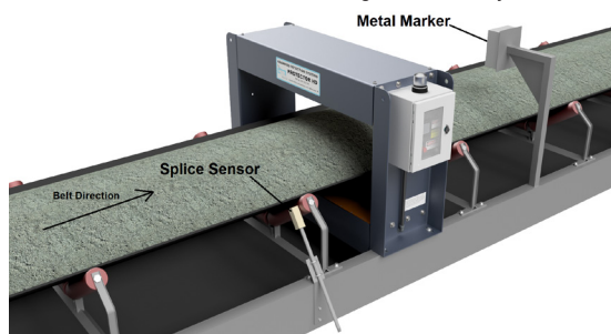
Protector HD Metal Detector on Trough Belt Conveyor
