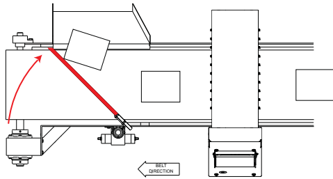
SWEEP ARM
