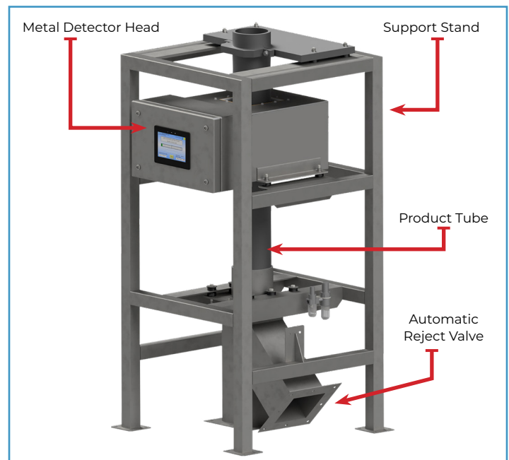
* Gravity Drop metal Detector System
