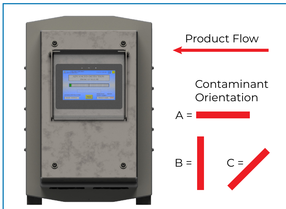
* Diagram of contaminant orientation
