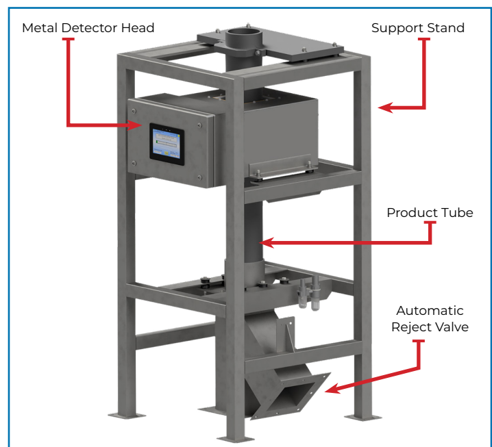
* Gravity Drop metal Detector System
